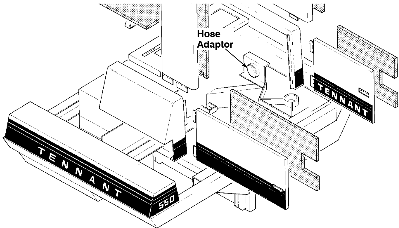
TRACTOR FRAME
