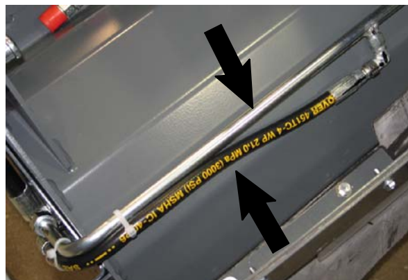
Install return tubing and drain hose on to scrub head and front brush motor
