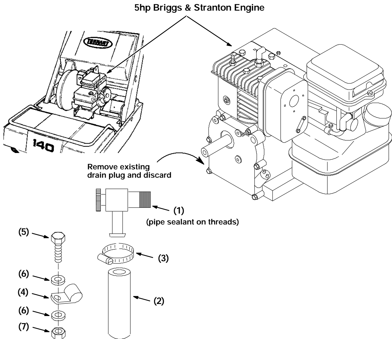
FIG. 1 - Engine And Drain Plug Assembly BILL OF MATERIALS FOR DRAIN PLUG KIT 23263
