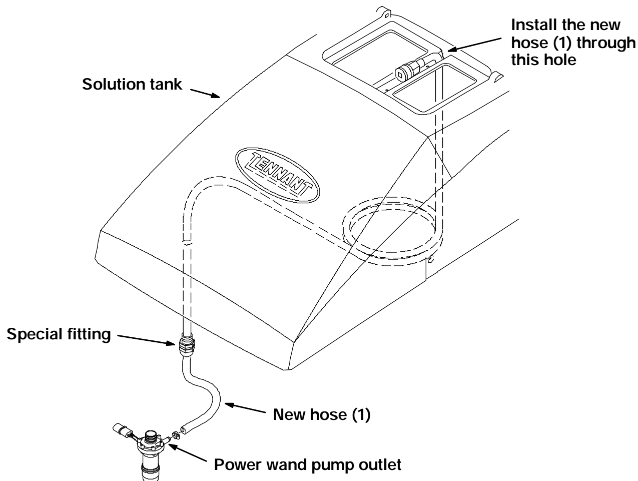
FIG. 1 - Power Wand Pump Hose
