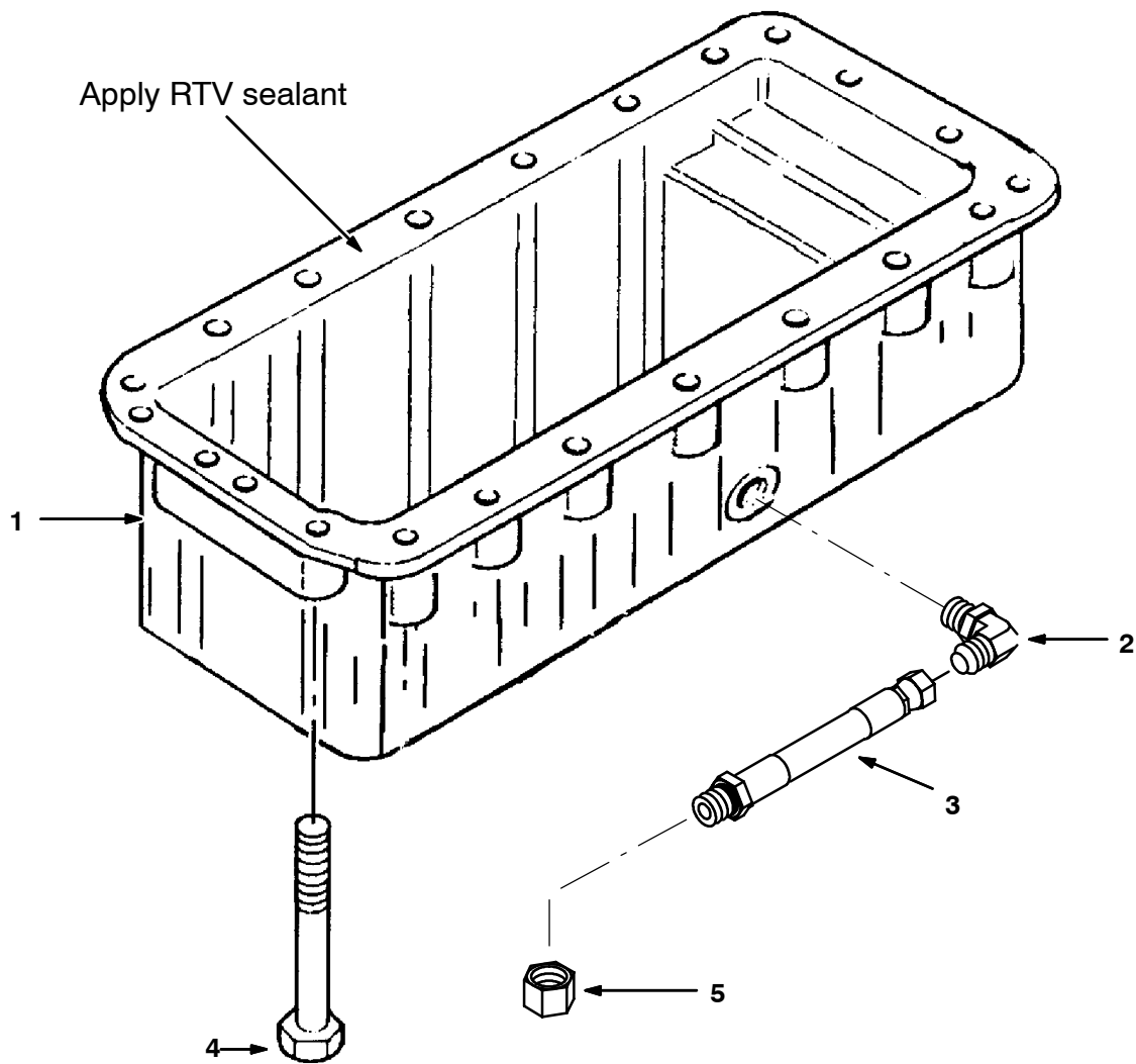
FIG. 1 - New Oil Pan Assembly
