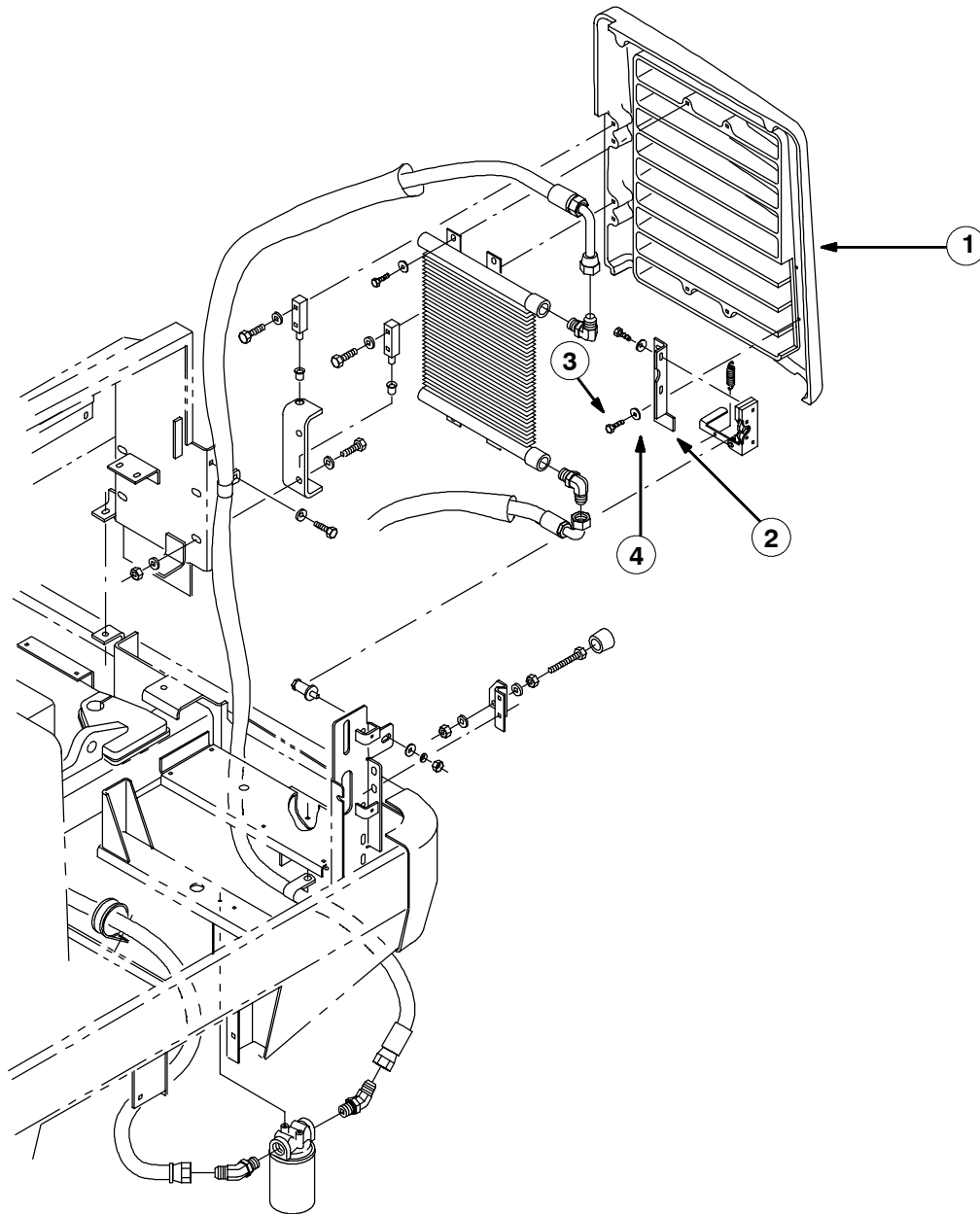
FIG. 1 - Rear LH Grille Door Installation
