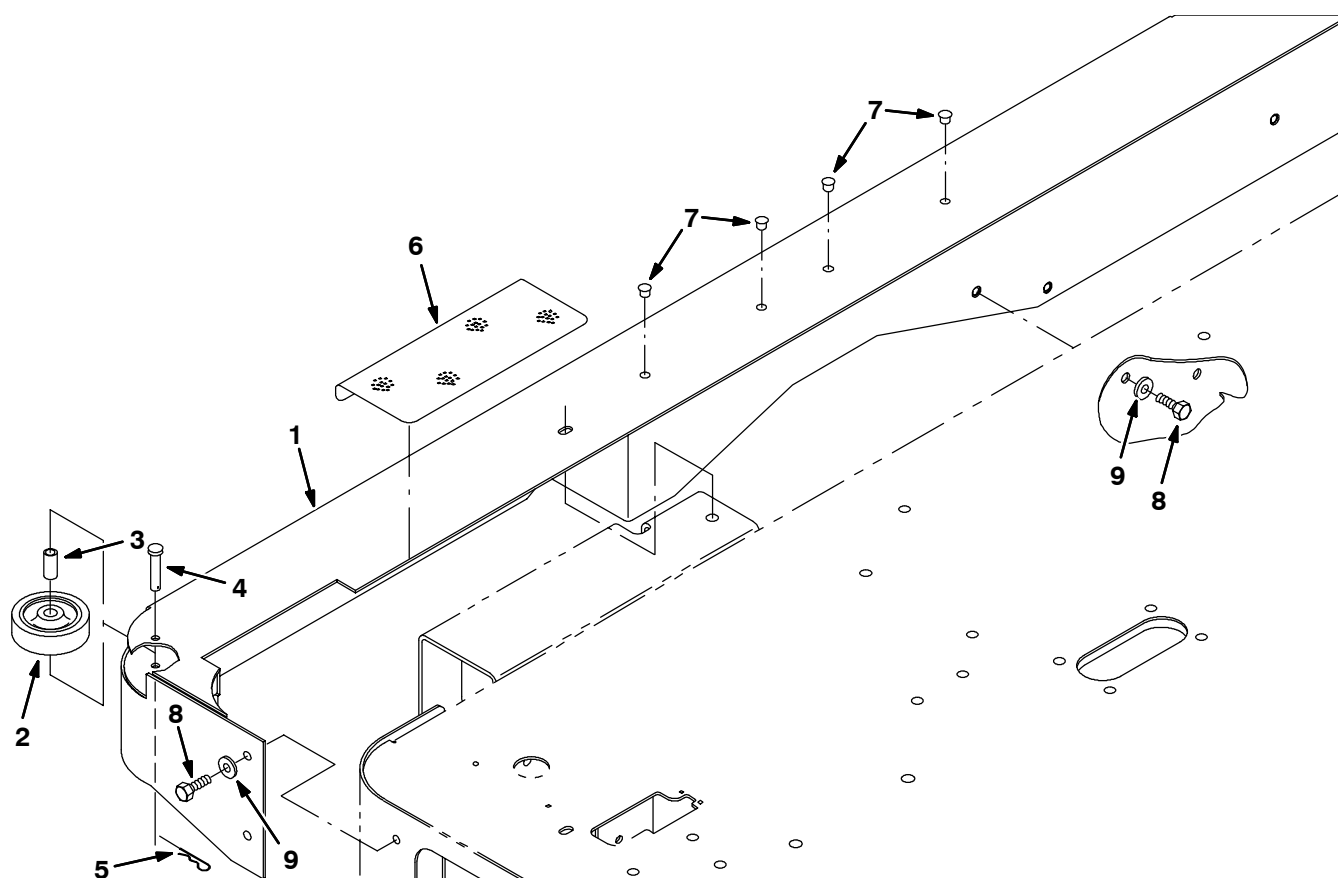
FIG. 3 - Side Brush Bumper Group
