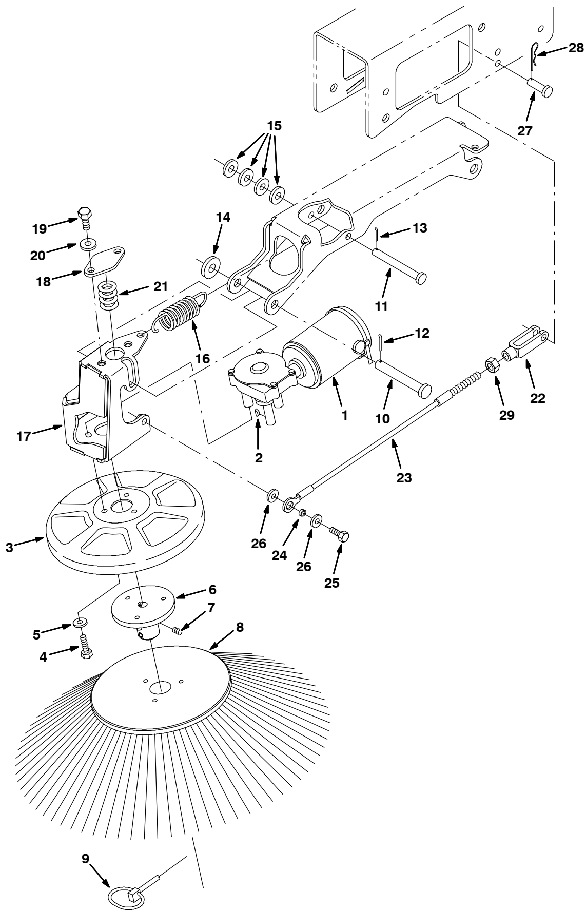
FIG. 2 - Side Brush Motor Group
