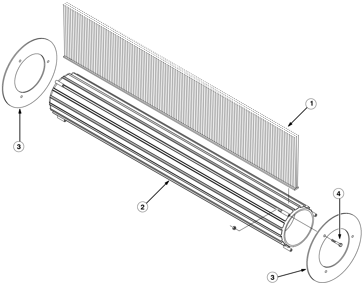
FIG. 1 - Strip Brush Replacement
