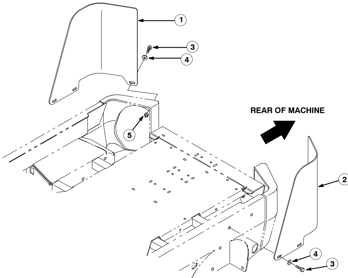
FIG. 1 - REAR BUMPER INSTALLATION
