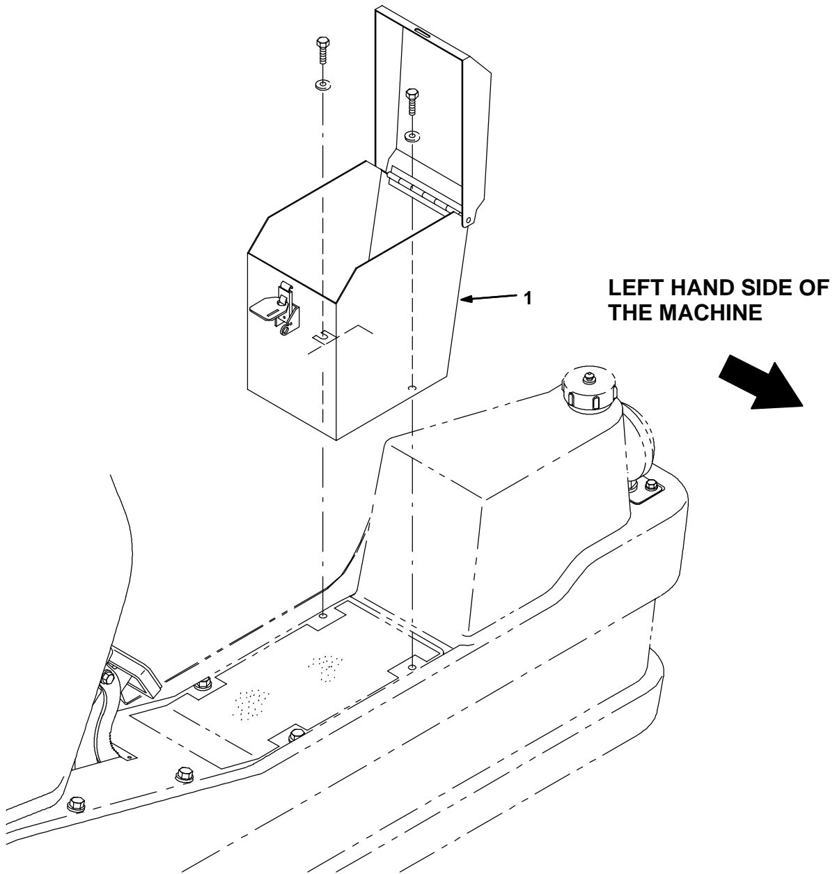
FIG. 1 - TOOL BOX KIT INSTALLATION
