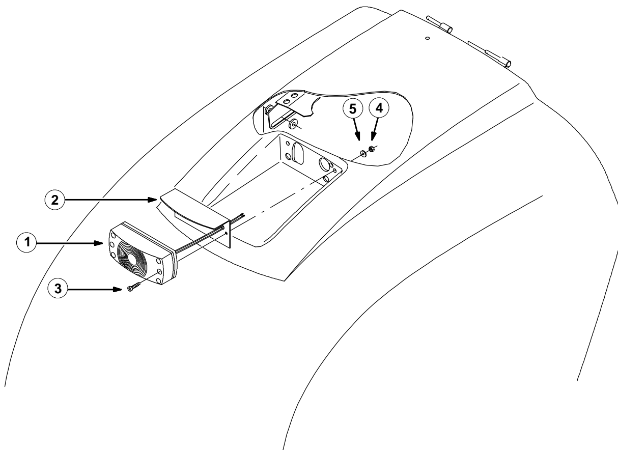
FIG. 2 - STROBE LIGHT INSTALLATION
