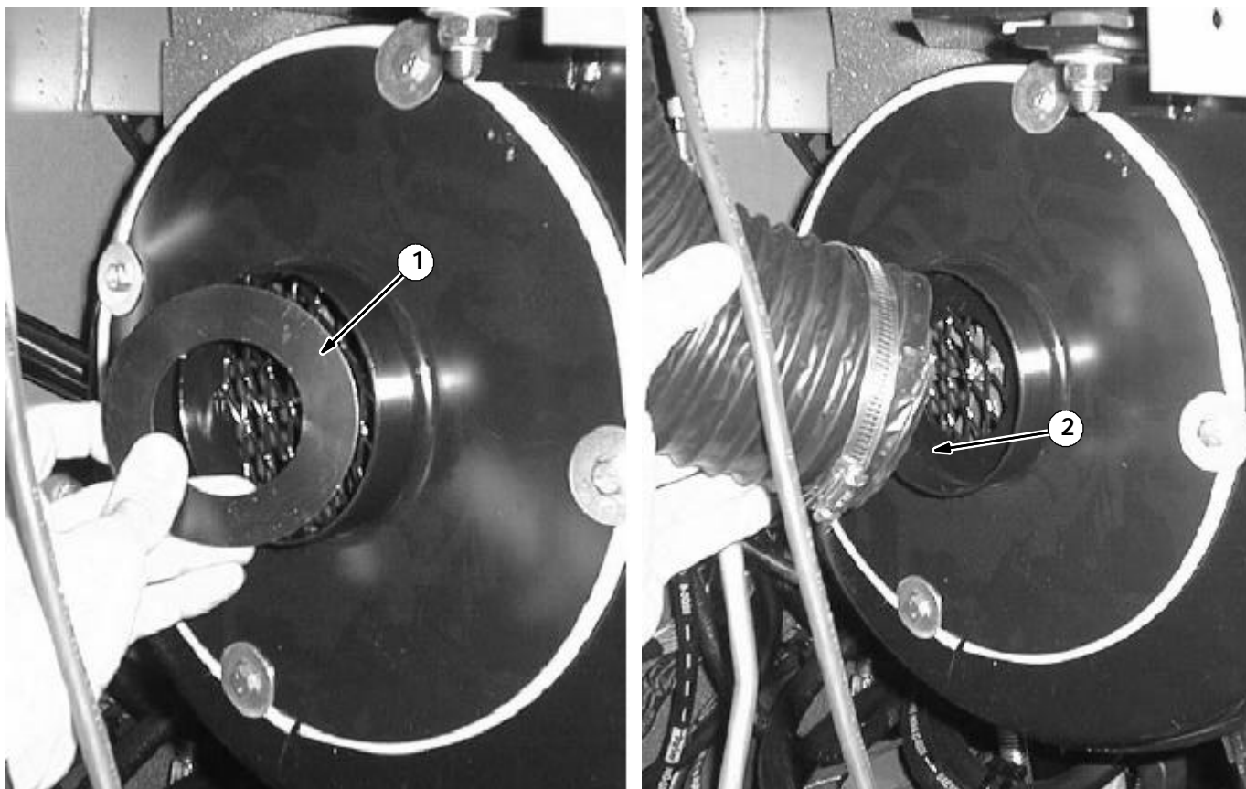
FIG. 1 - RESTRICTOR RING INSTALLATION
