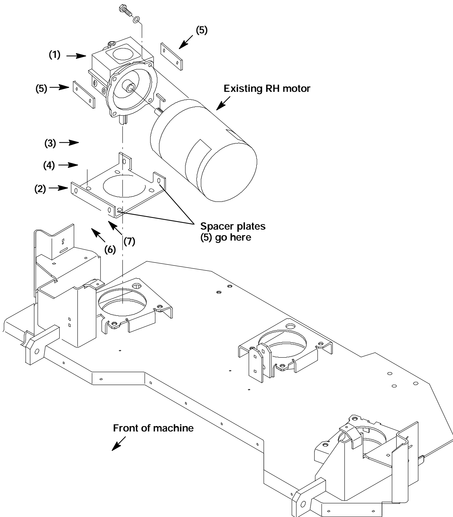
FIG. 1 - MAX PRO 1200 Scrub Head (RH gear box only)
