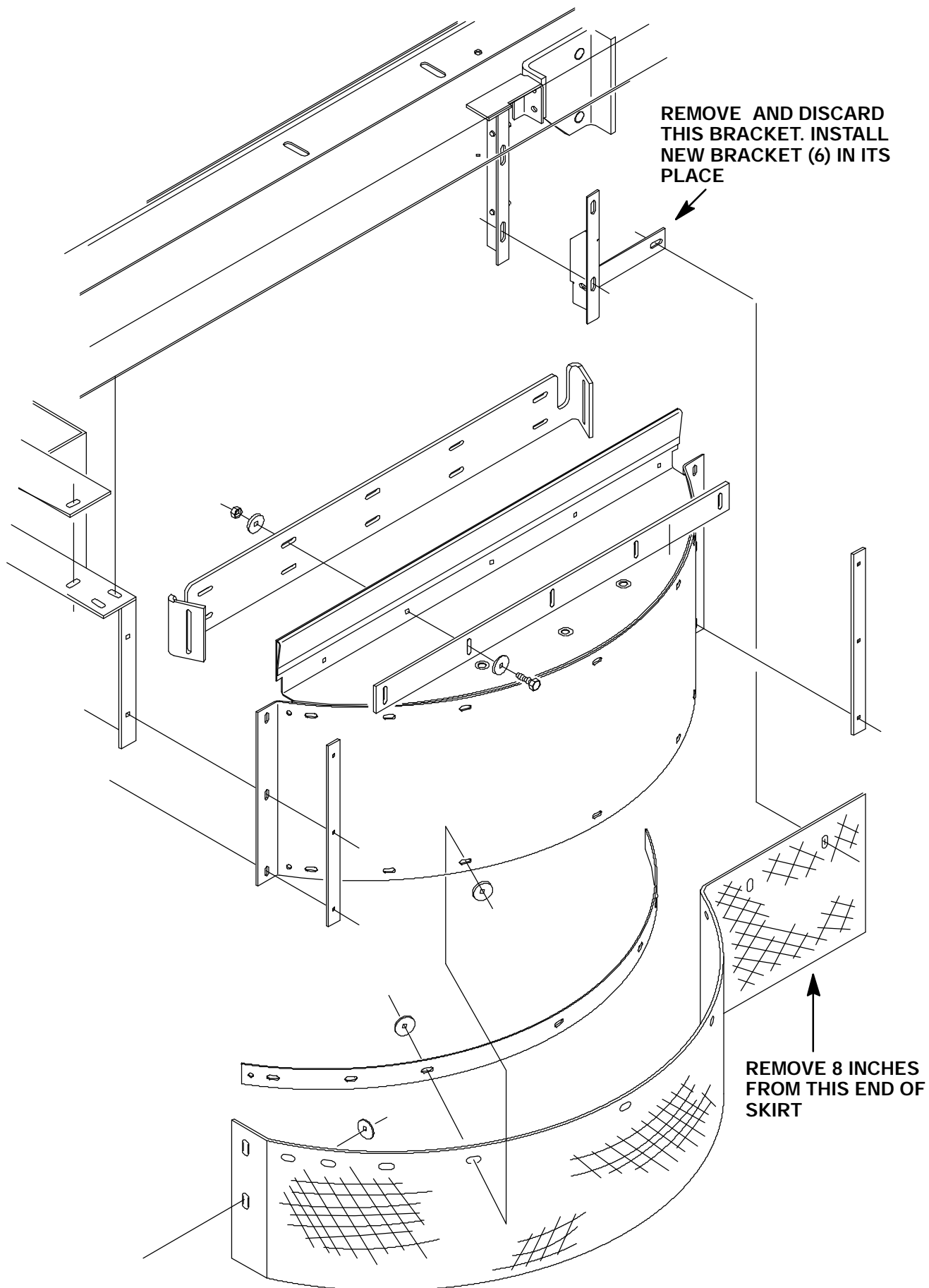
FIG. 1 - Left Hand Side Brush Skirt Rework And LH Bracket Removal
