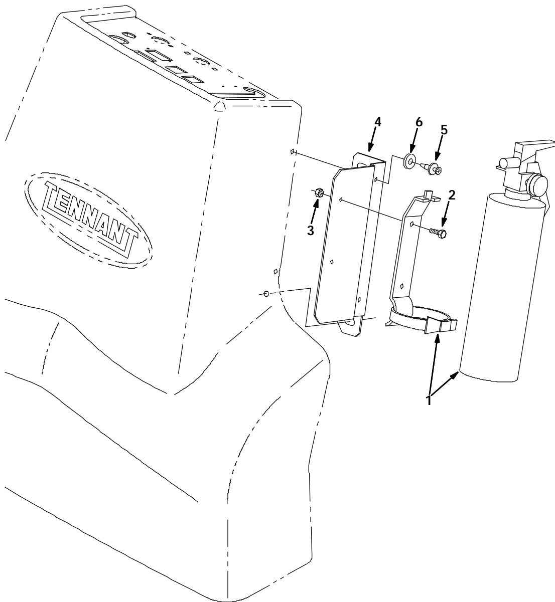
FIG. 1 - FIRE EXTINGUISHER KIT INSTALLATION
