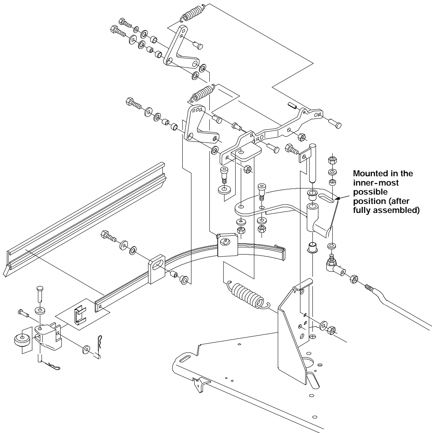
FIG. 2 - Installation of Side Squeegee Stabilizing Rod on Right Hand Side of Machine BILL OF MATERIALS FOR KIT NUMBER 365144
