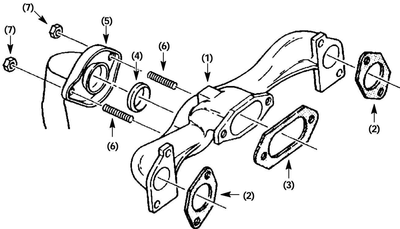
FIG. 1 - Exhaust Manifold, Gaskets, And Hardware
