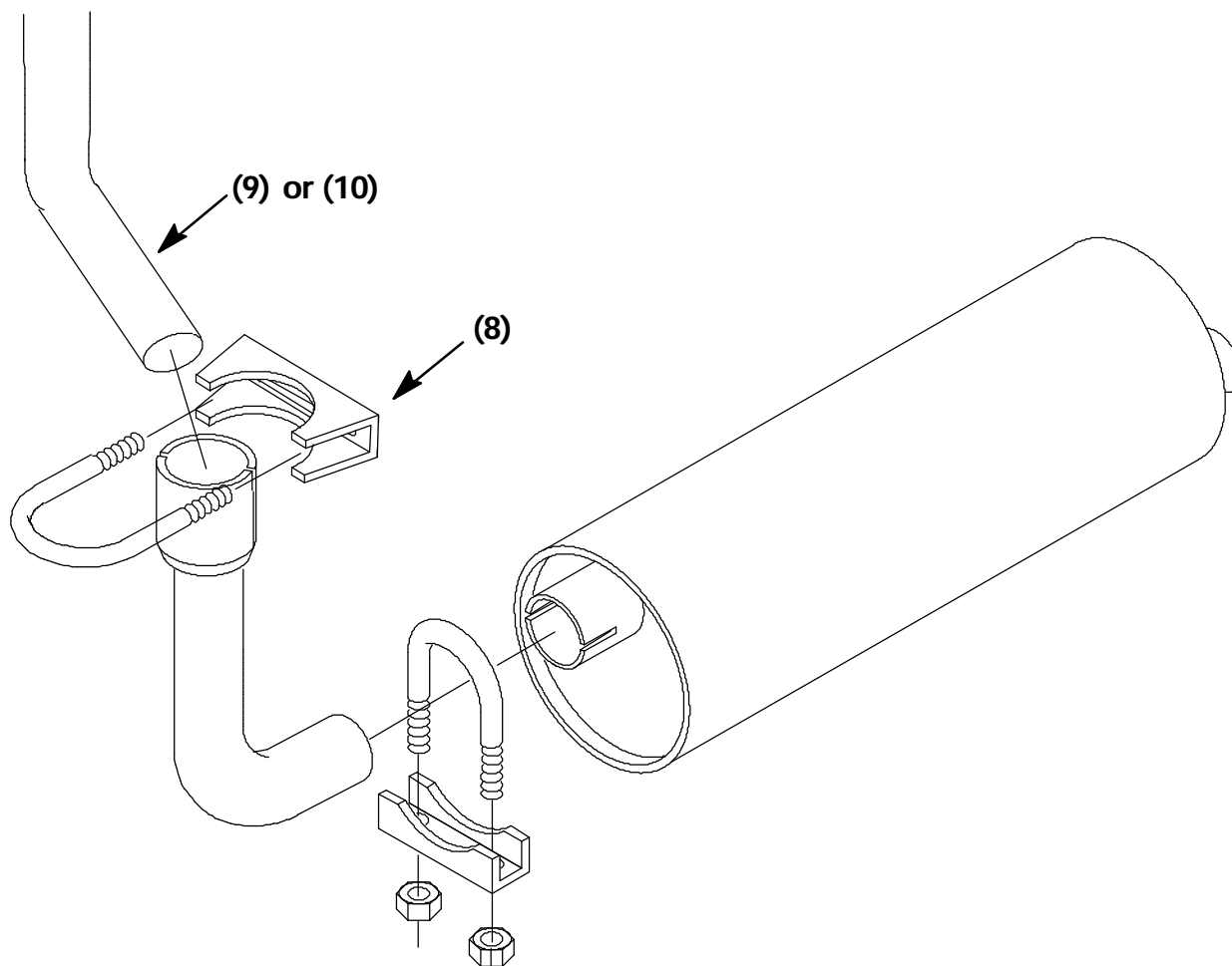
FIG. 2 - Exhaust Pipes And Muffler
