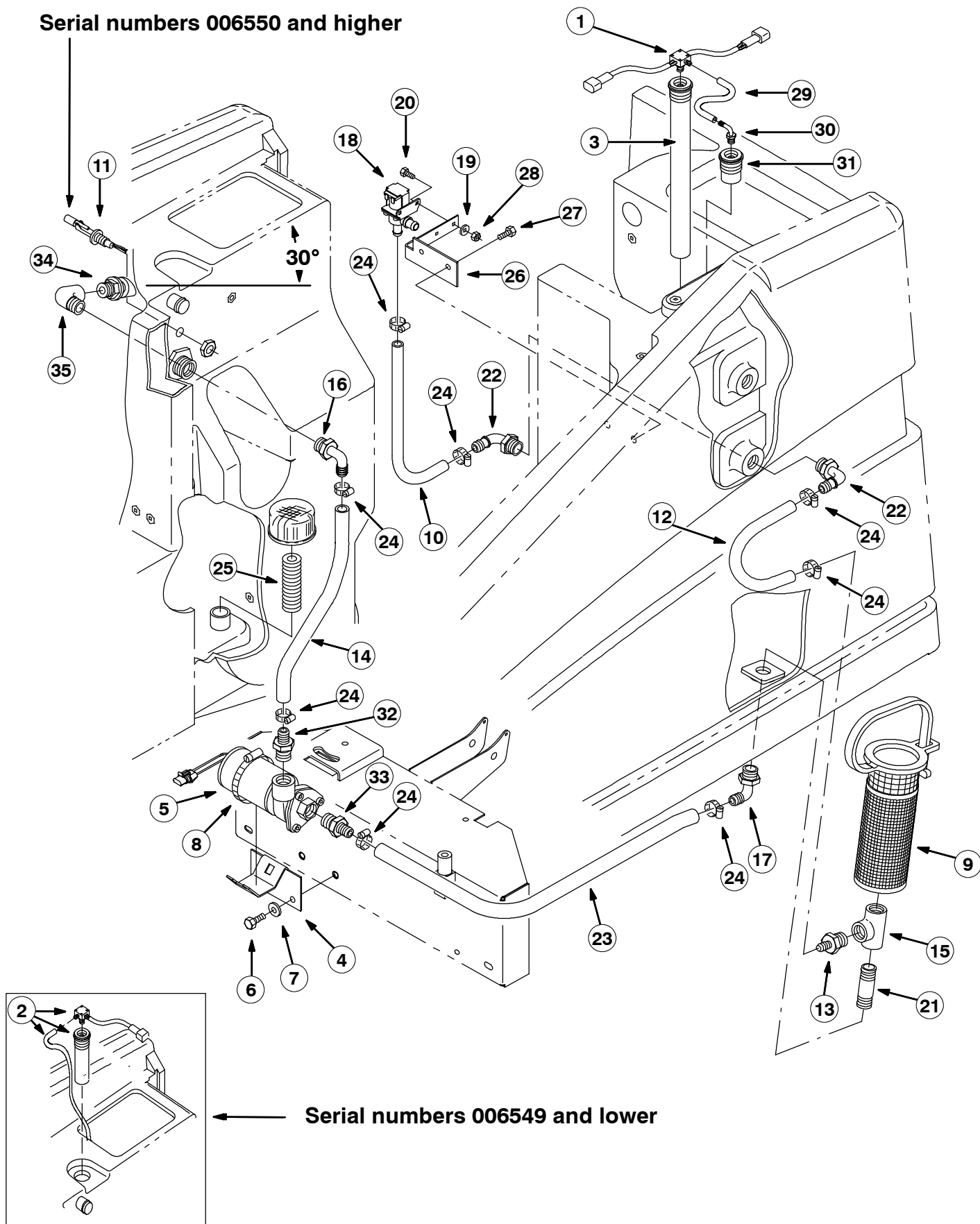
FIG. 2 - ES™ Pump Group
