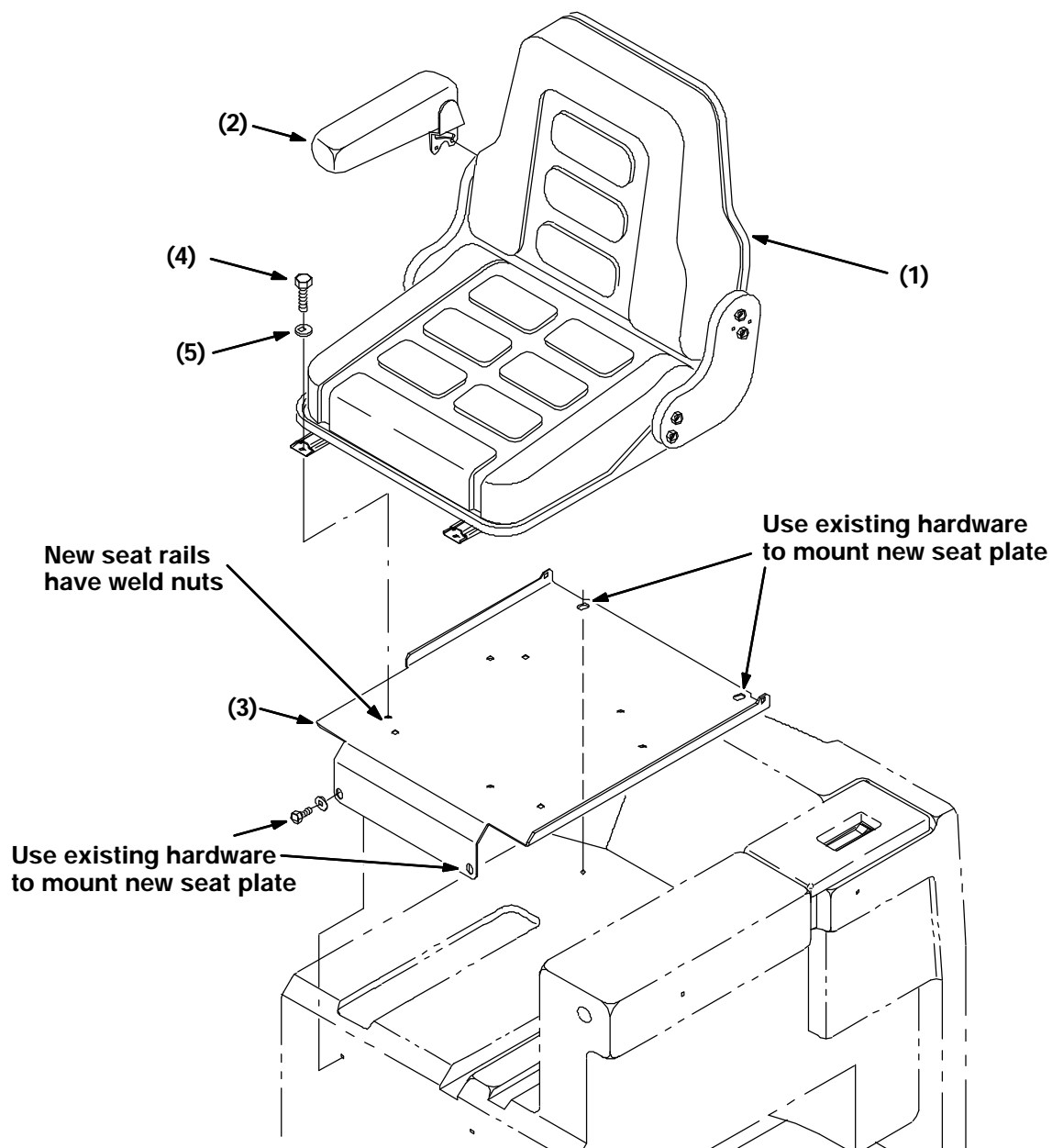
FIG. 1 - Installation of Grammer Seat
