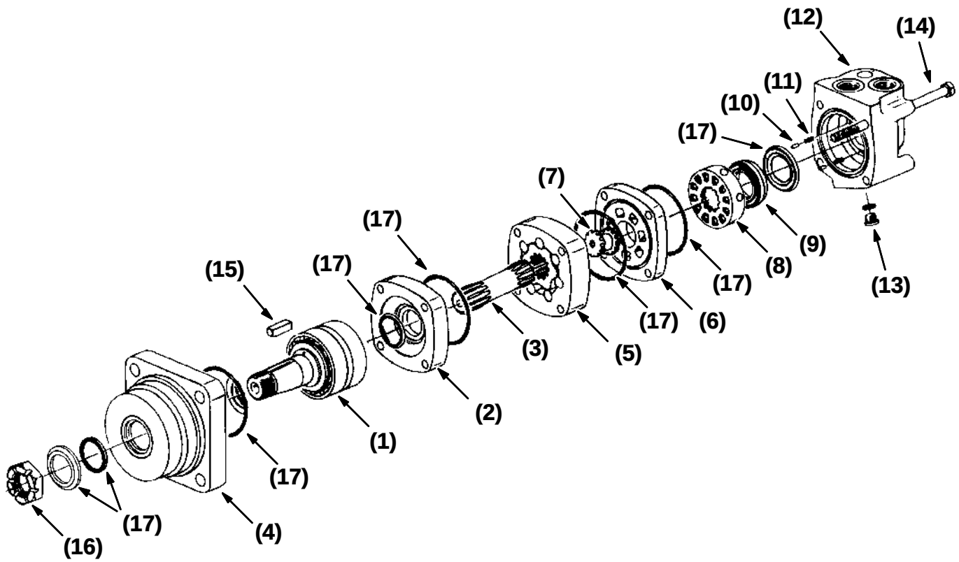
FIG. 1 - MOTOR PARTS BREAKDOWN (PART # 361025)
