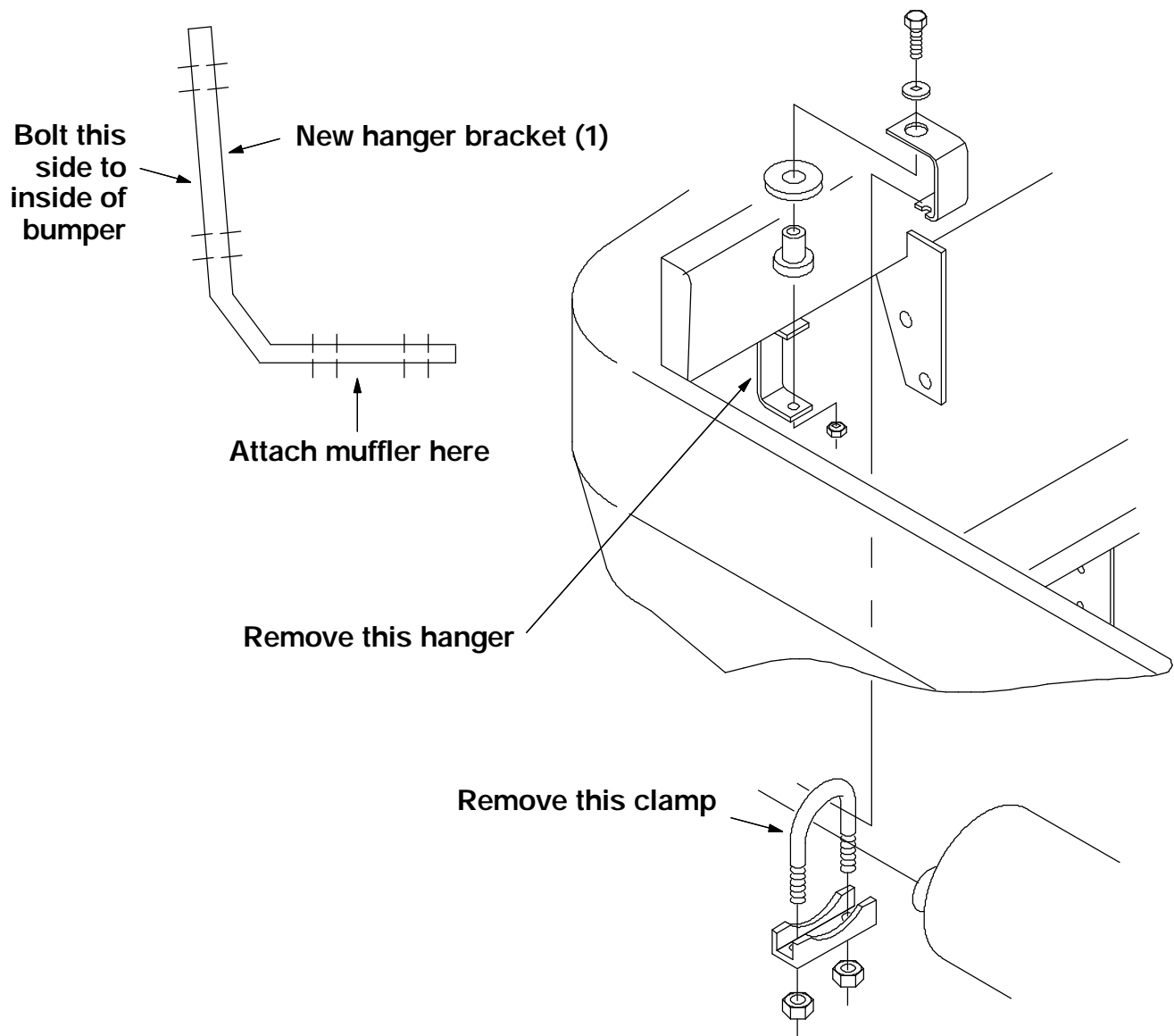
FIG. 1 - 385DLH Muffler, Tail Pipe, And Hanger Assembly
