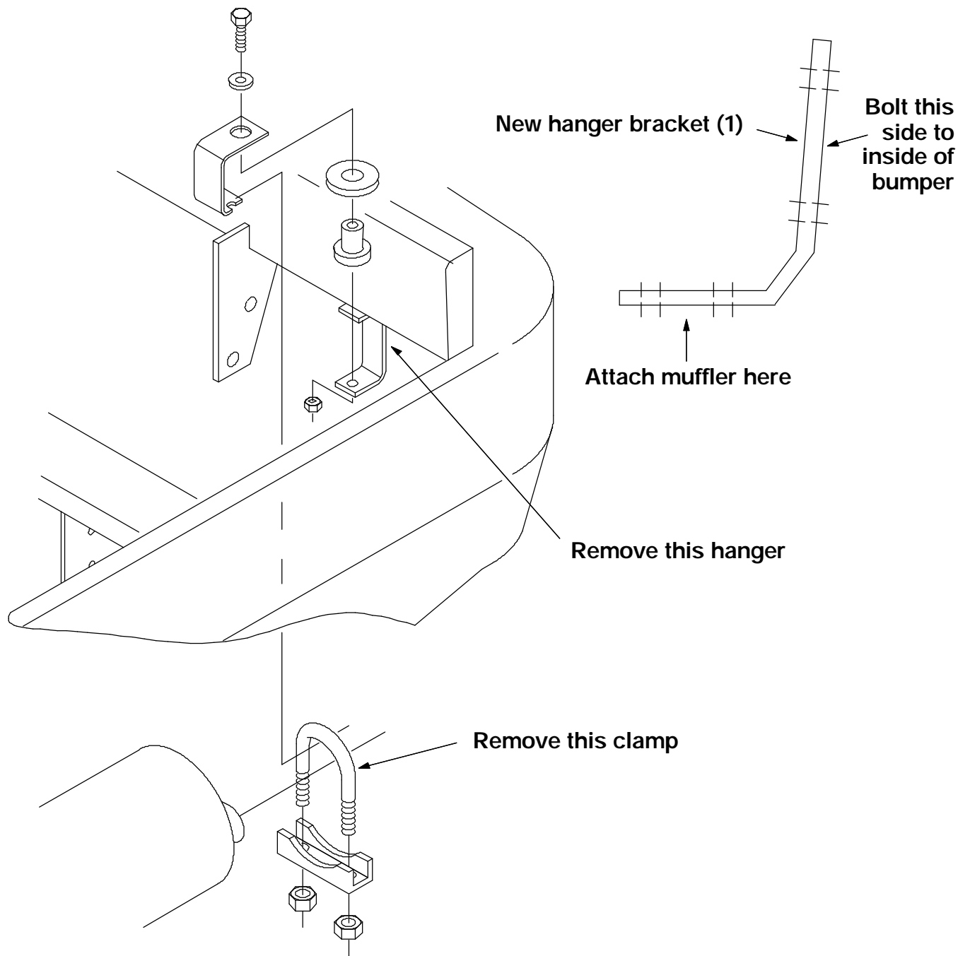
FIG. 2 - 355-385 Muffler, Tail Pipe, And Hanger Assembly
