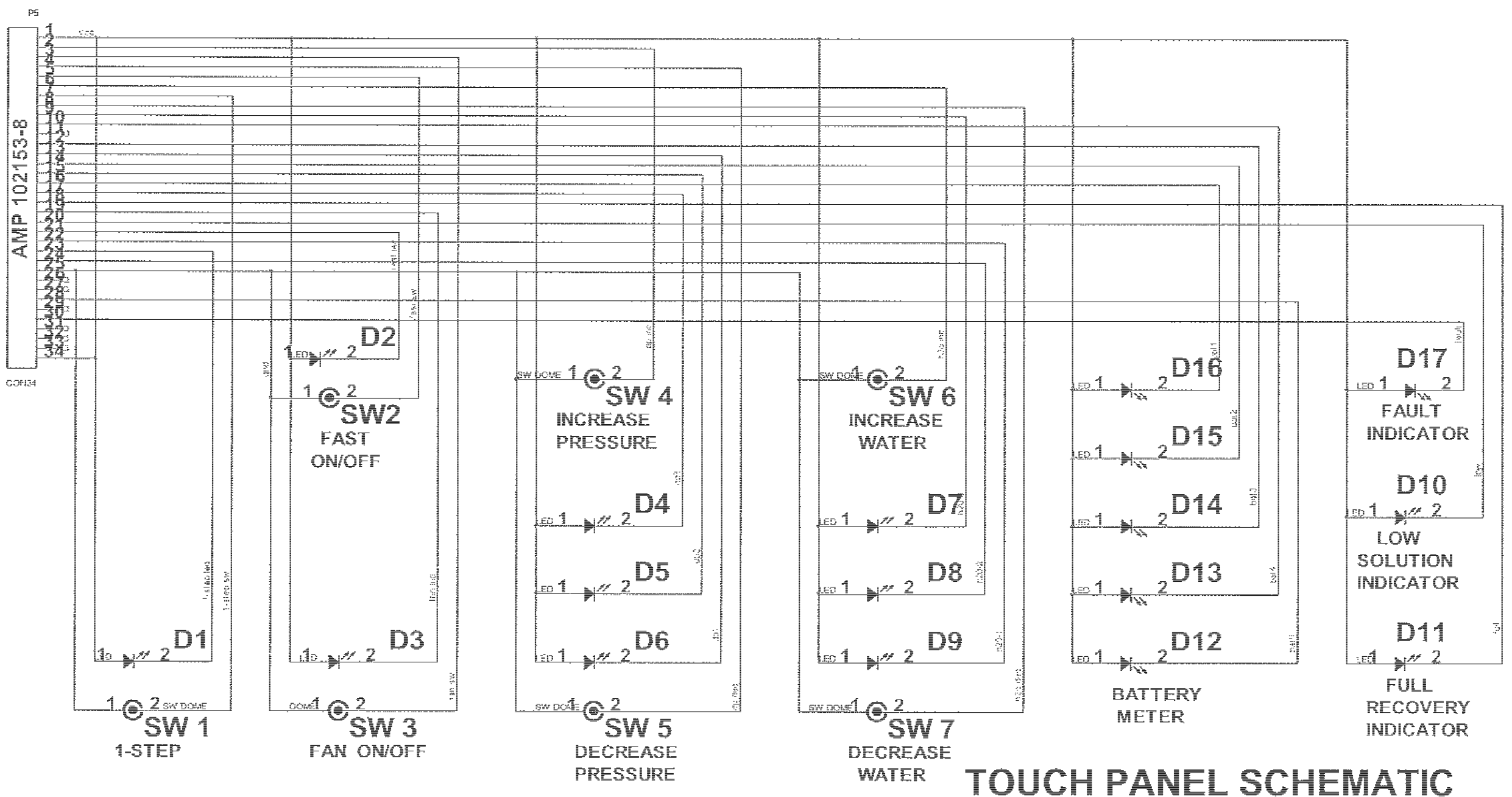
TOUCH PANEL SCHEMATIC
